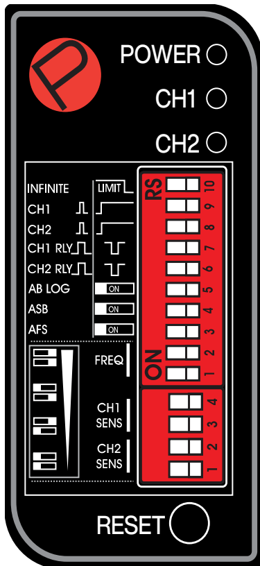
Figure 3. LC20-2 Faceplate
